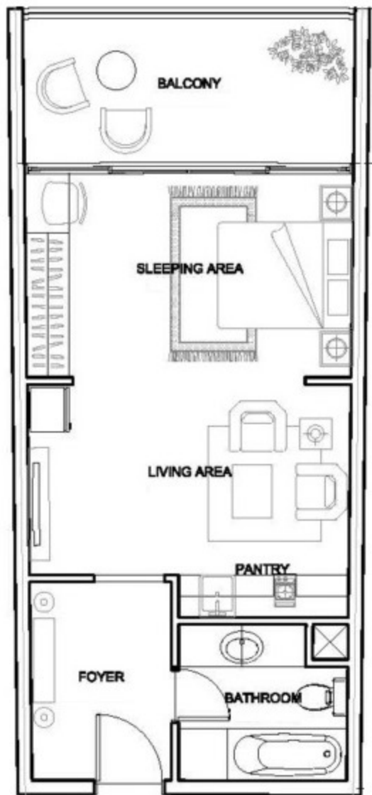
STUDIO TYPE. PLAN (TYPE-K)
