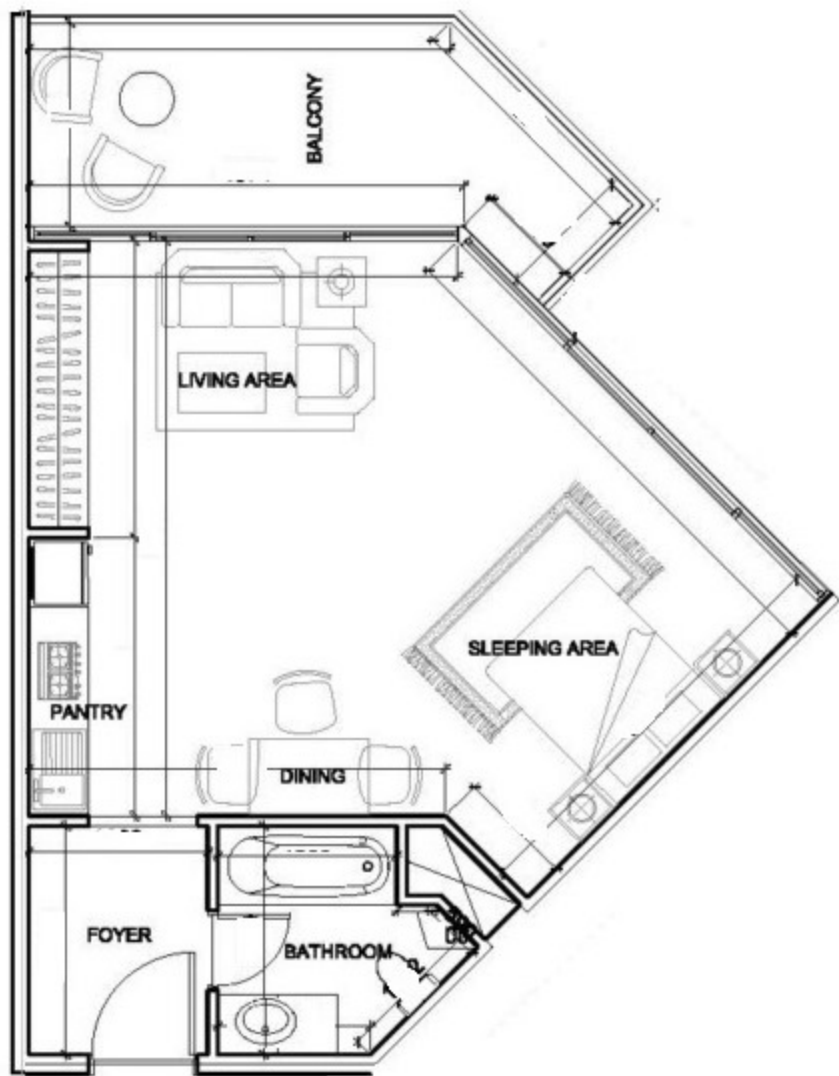
STUDIO TYPE. PLAN (TYPE-E)
